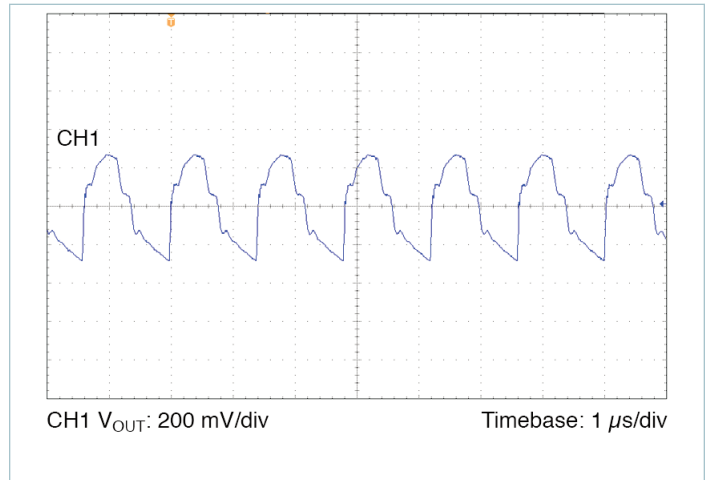
Figure 16 — Output voltage ripple, V_{IN} = 28\text{ V} , V_{OUT} = 15.0\text{ V} , C_{OUT\_EXT} = 680\ \mu\text{F} , R_{LOAD} = 0.701\ \Omega
