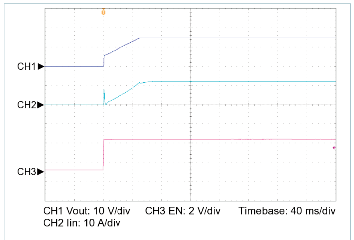
Figure 14 — Startup from EN, V_{IN} = 28\text{ V} , C_{OUT\_EXT} = 6800\ \mu\text{F} , R_{LOAD} = 0.701\ \Omega
